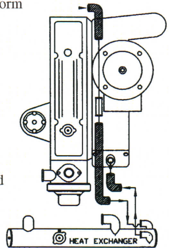
SEAWATER FLOW SCHEMATIC
