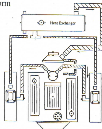
MERCUISER 7.4 ENGINES COOLANT WATER SCHEMATIC FULL SYSTEM
